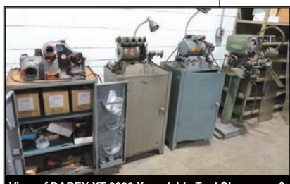
View of DAREX XT 3000 Xpandable Tool Sharpener & Black Diamond Drill Grinders
